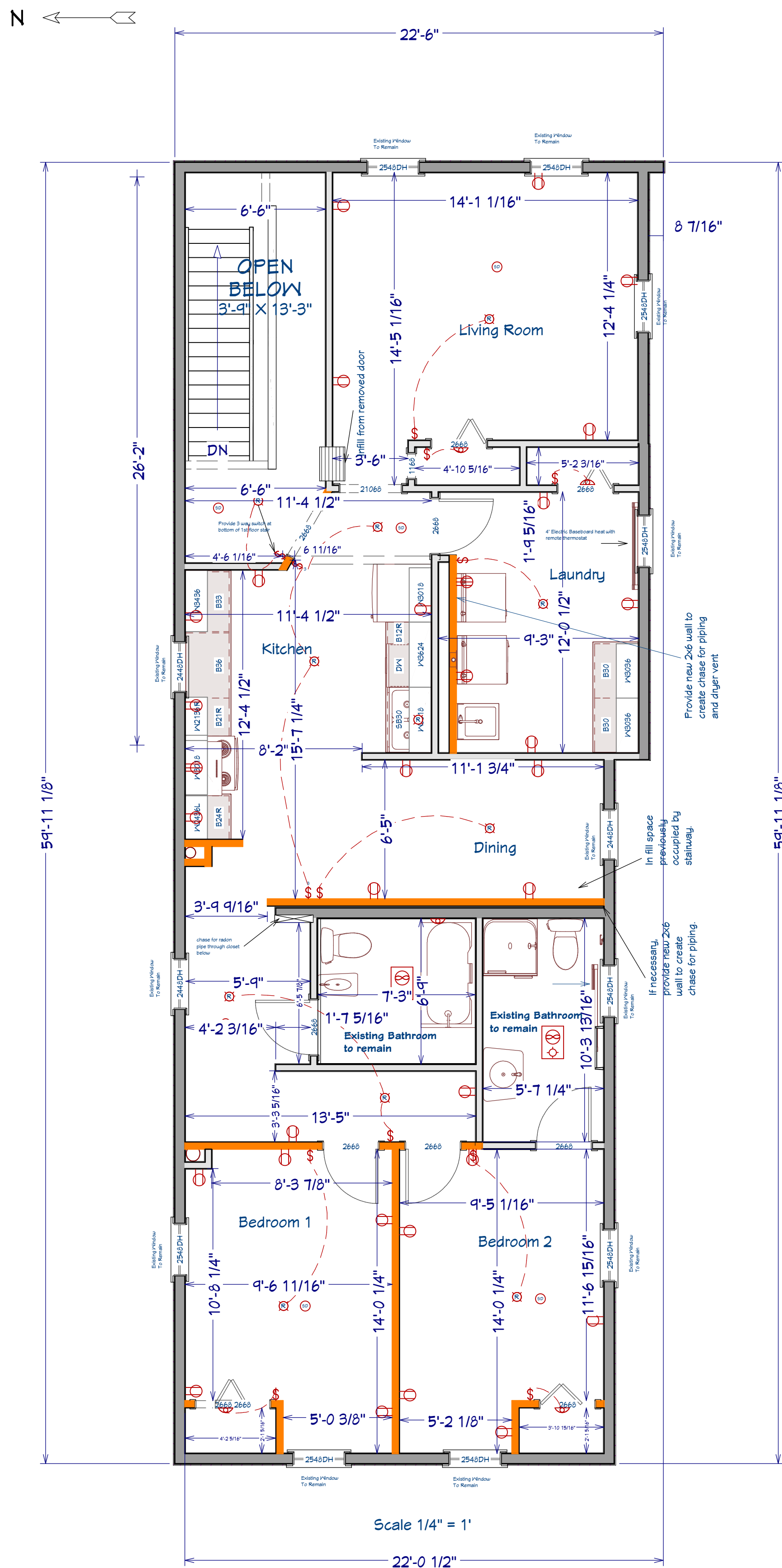
39 NORTH 12TH STREET PROPOSED 2ND FLOOR PLAN 1,100 SF
