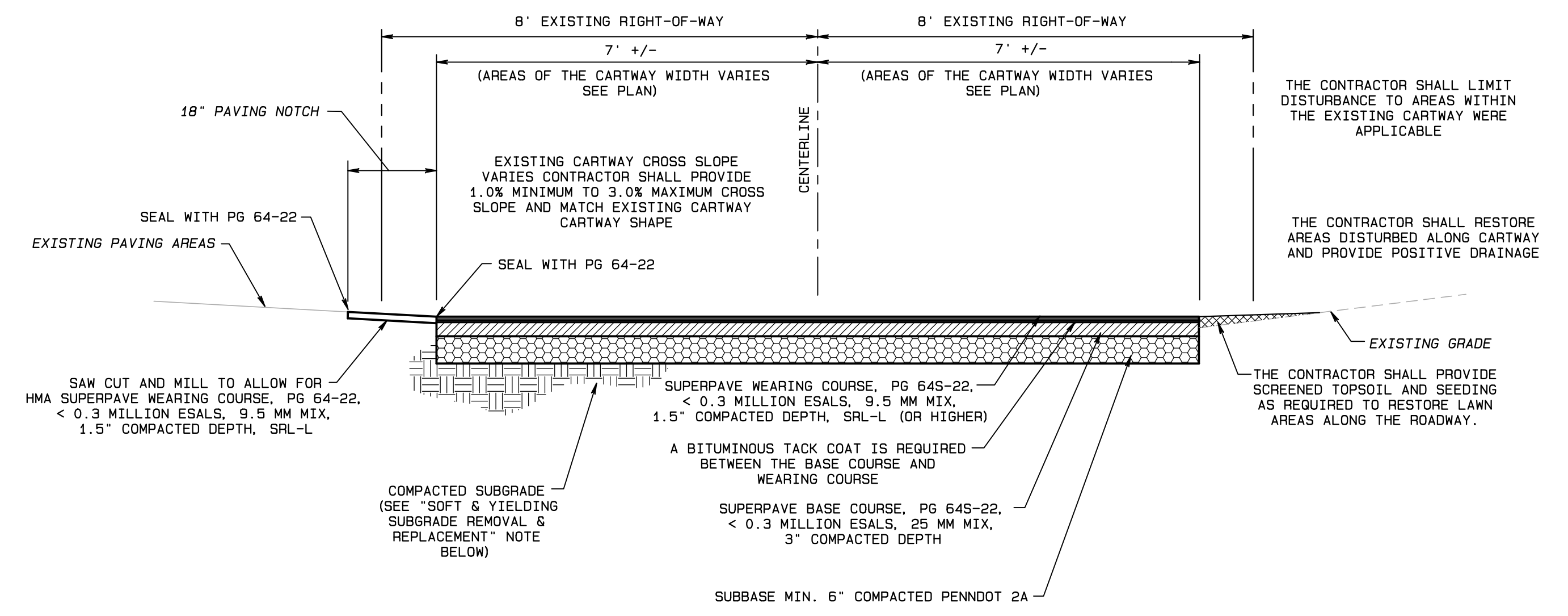
FULL DEPTH REPLACEMENT SECTIONS NOT TO SCALE
