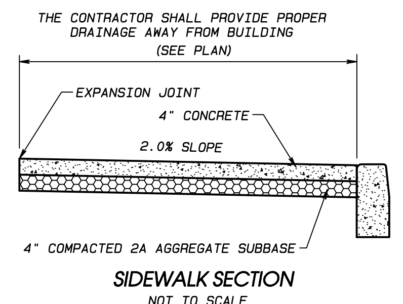
SIDEWALK SHALL BE CONSTRUCTED PER PENNDOT PUB. 408 SECTION 676 AND PUB. 72M.
