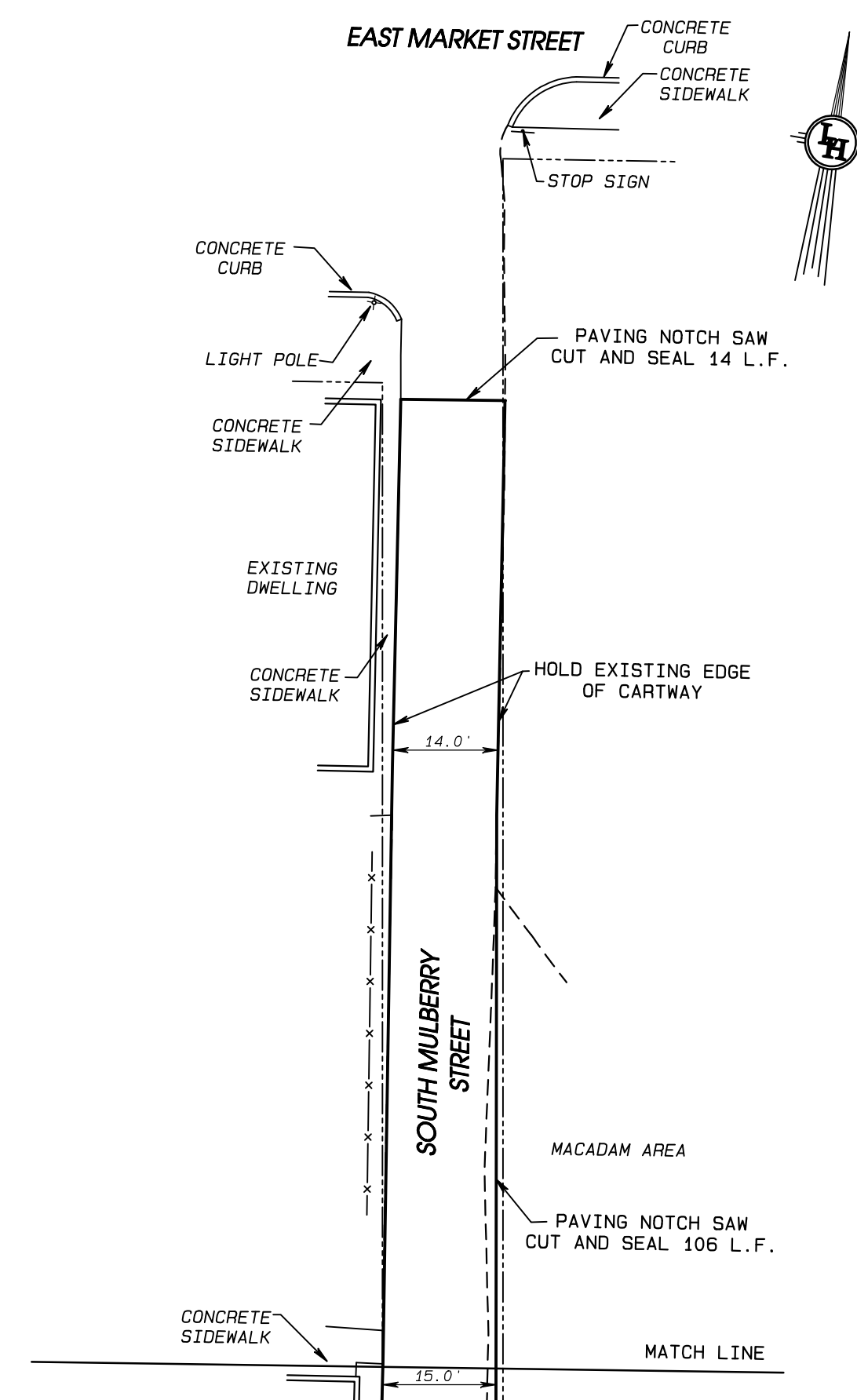
IMPROVEMENT PLAN HORIZONTAL SCALE 1" = 20'
