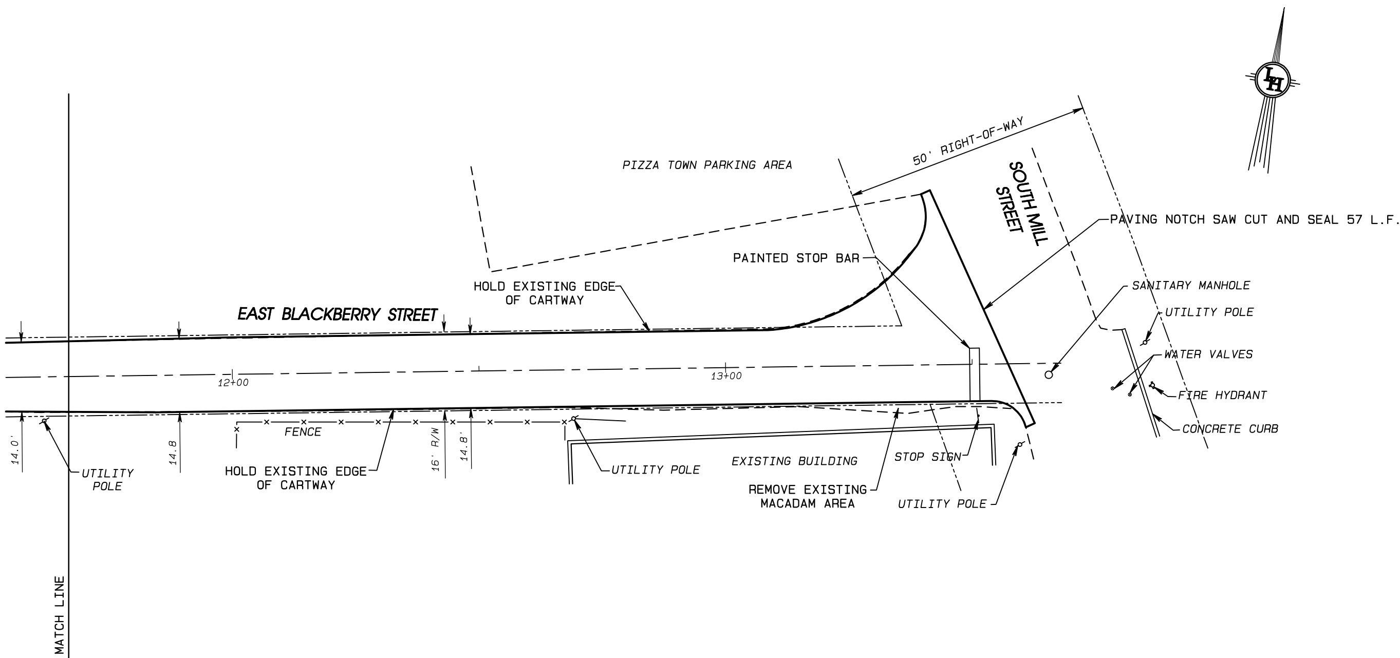
IMPROVEMENT PLAN HORIZONTAL SCALE 1" = 20'
